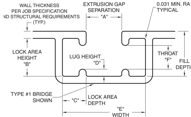
Figure 1: Cavity recommendations
